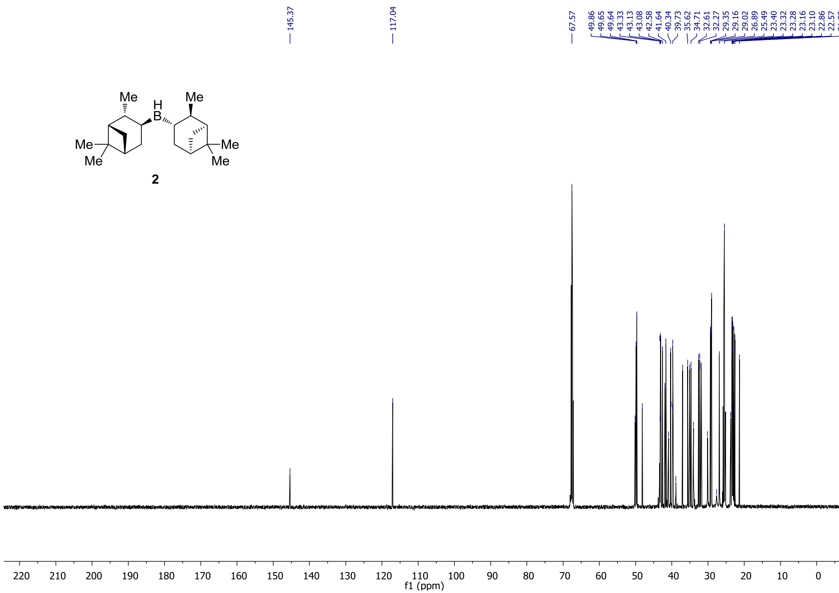
^{13}\text{C} NMR spectrum (125 MHz, anhydrous d_8 -THF) of compound 2
